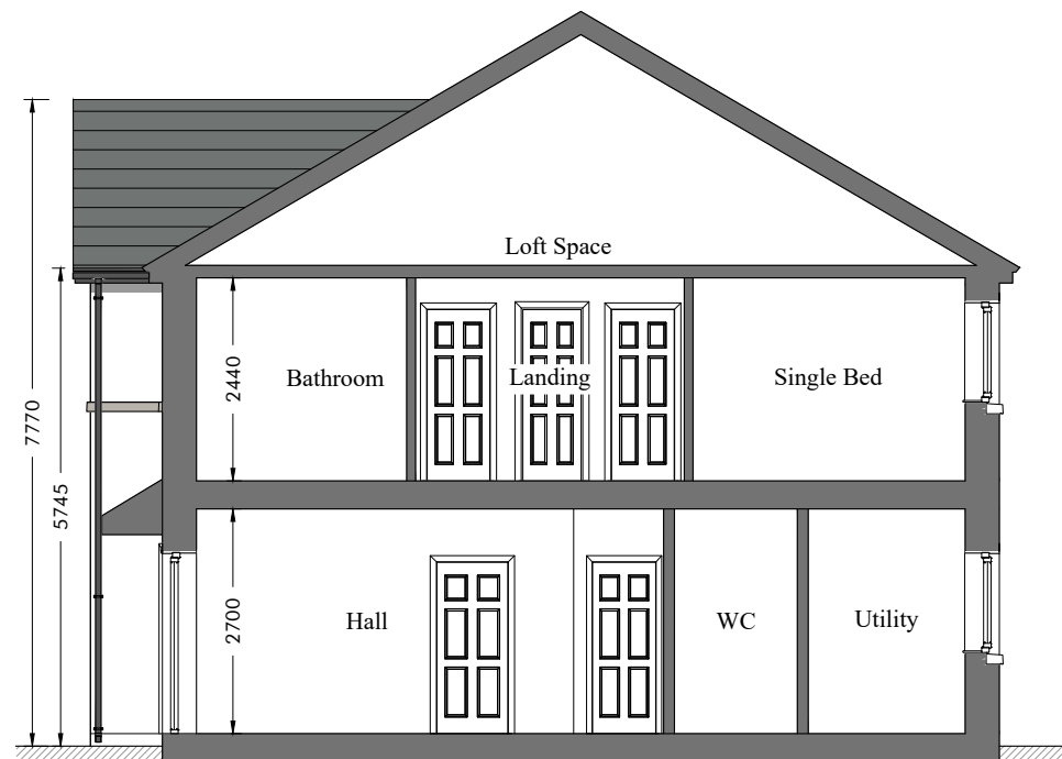
HOUSE TYPE: B SECTION 3-3_STYLE 01 CLASSIC
